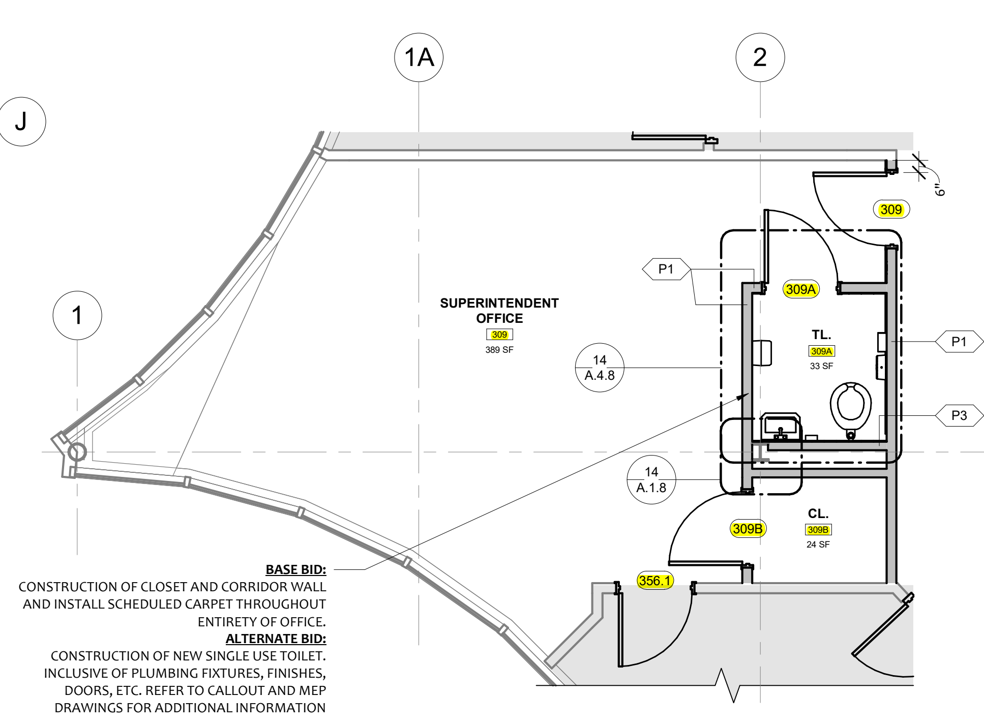
③ ALTERNATE BID - ENLARGED PLAN - THIRD FLOOR SUPERINTENDENT OFFICE 1/4" = 1'-0"
